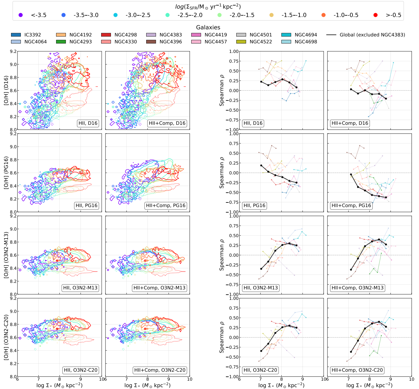
Figure 6. Comparison of the rMZR (left two columns) and the mass-dependent Spearman rank correlation coefficient \rho between \Delta[\text{O}/\text{H}] and \Delta\log_{10}\Sigma_{\text{SFR}} (right two columns) for four gas-phase metallicity calibrations: D16 (top row), Scal-PG16 (second row), O3N2-M13 (third row), and O3N2-C20 (bottom row). Columns 1 and 3 use only HII -classified star-forming spaxels, whereas Columns 2 and 4 use the more inclusive HII+Comp selection (see the BPT demarcation in Figure 1). The rMZR panels are colour-coded by \log_{10}\Sigma_{\text{SFR}} as in Figure 3. The Spearman panels show \rho(\Sigma_*) measured in discrete \Sigma_* bins for individual galaxies (coloured curves) and for the ensemble sample (black curve; excluding NGC 4383), following Figure 5. The parameter spaces occupied by NGC 4383 are indicated by dotted contours/curves in each corresponding panel.
